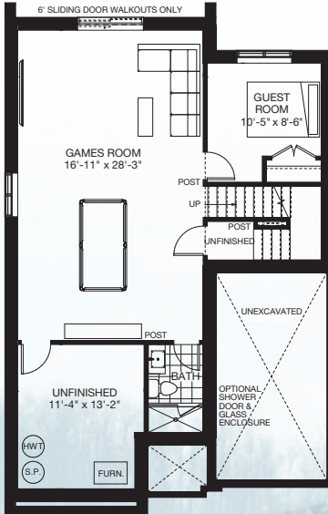
OPT. FINISHED BASEMENT (755 SF)
