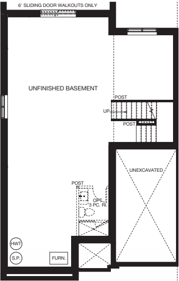
UNFINISHED BASEMENT
